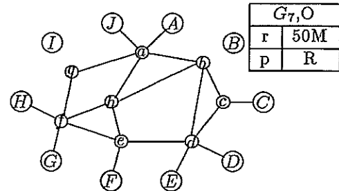
Figure 1: One-to-Many Connection
