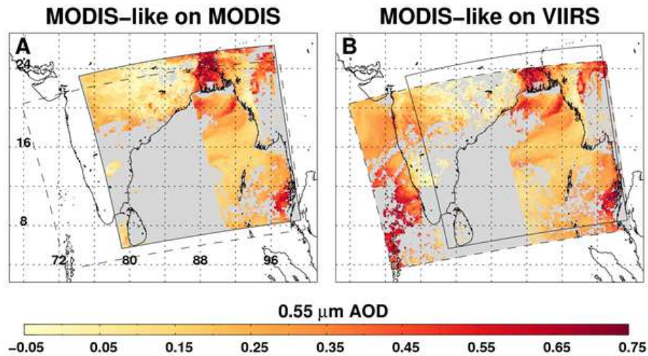
Figure 6. QA-filtered AOD at 0.55 μm over the Bay of Bengal on 5 March 2013 at 07:35, retrieved with MODIS-like algorithm on (a) MODIS (at 10 km) and (b) VIIRS (at 7.5 km). This is the same observational overlap as pictured in Fig. 2.
