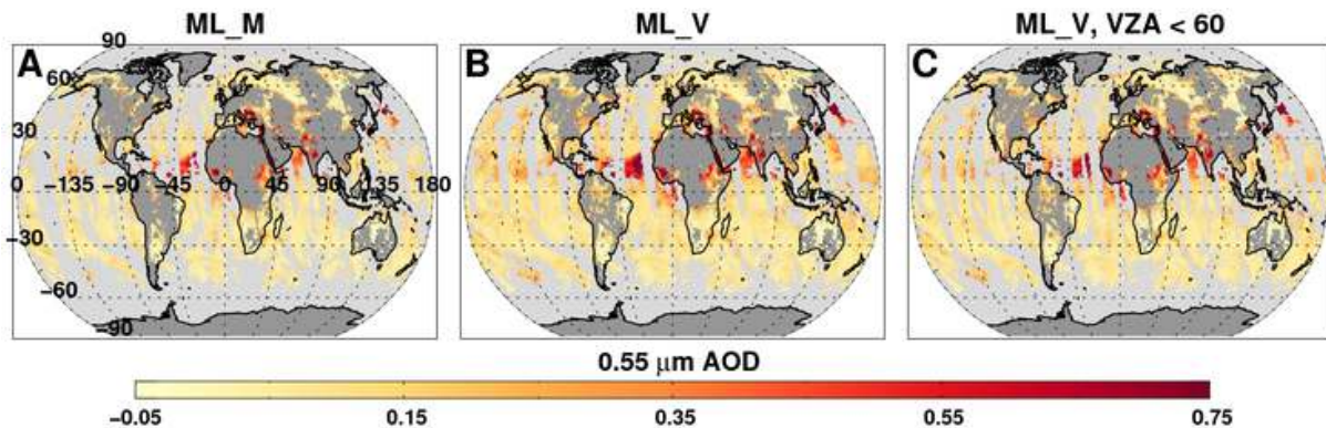
Figure 7. AOD at 0.55 μm, retrieved using MODIS-like algorithm on MODIS (a) and VIIRS (b), created from all orbits during 29 May 2013 (see Fig. 1). (c) approximates the MODIS coverage by reducing the VIIRS swath to sensor view angles less than 60°.
