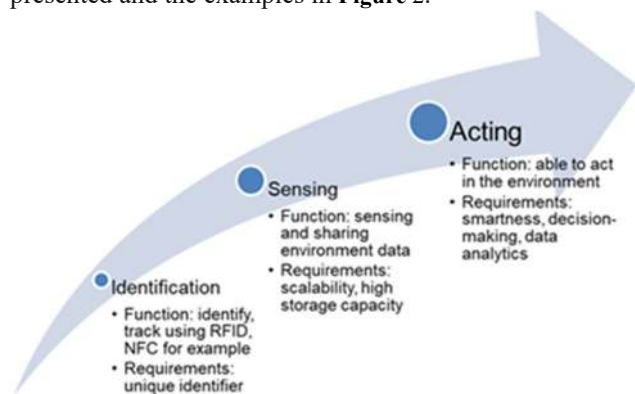
Figure 2 IoT evolution.
