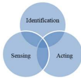
Figure 3 IoT behaviors.
