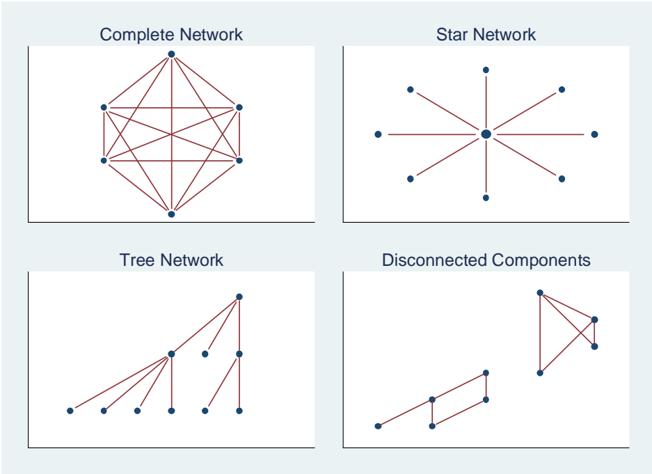
Figure 3: Basic types of (undirected) networks
