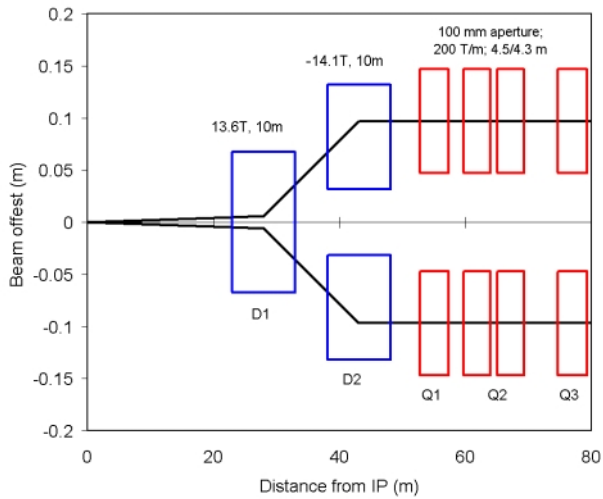
Figure 2: Dipoles-first IR.
