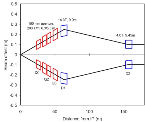
Figure 5: Quadrupole-first IR with large crossing angle.
