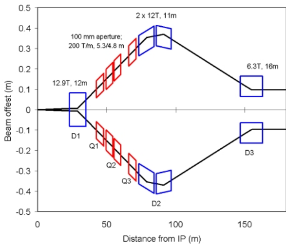
Figure 3: IR with quads between the separation dipoles.
