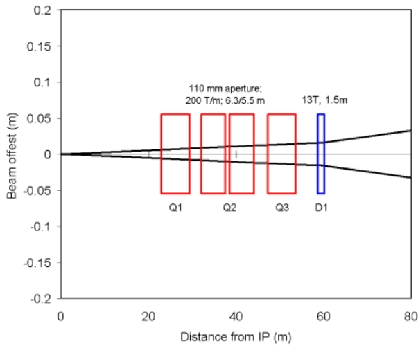
Figure 1: Quadrupole-first IR.
