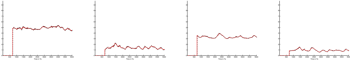
(i) Trend of \beta_{x_3}^{x_1} (red -) and 25Te forecast (black --) (j) Trend of \beta_{x_3}^{x_2} (red -) and 25Te forecast (black --) (k) Trend of \beta_{x_3}^{x_4} (red -) and 25Te forecast (black --) (l) Trend of \beta_{x_3}^{x_5} (red -) and 25Te forecast (black --)
