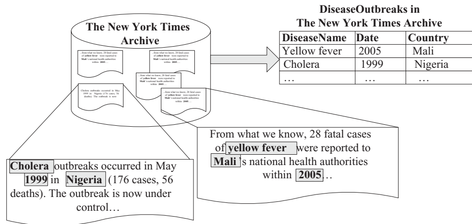
Fig. 1. Extracting DiseaseOutbreaks tuples.
