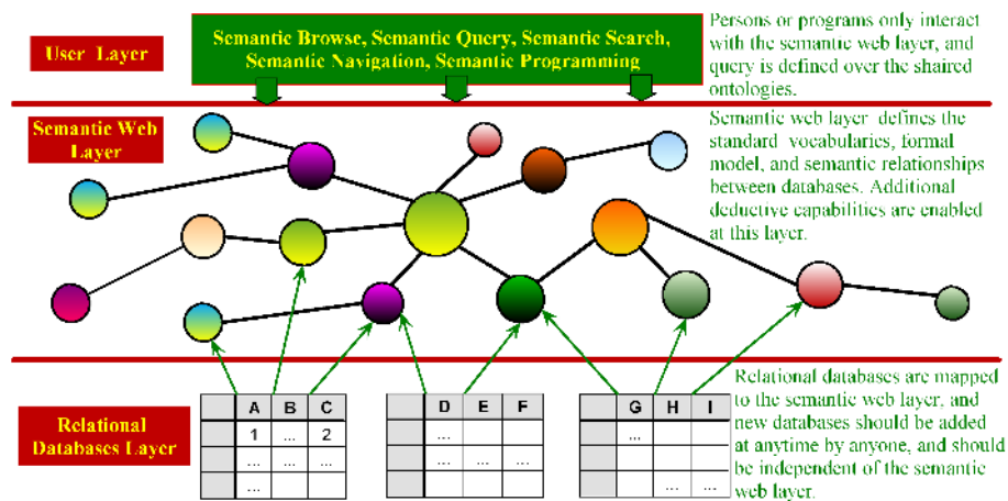
Fig. 1. Towards a semantic web of relational databases
