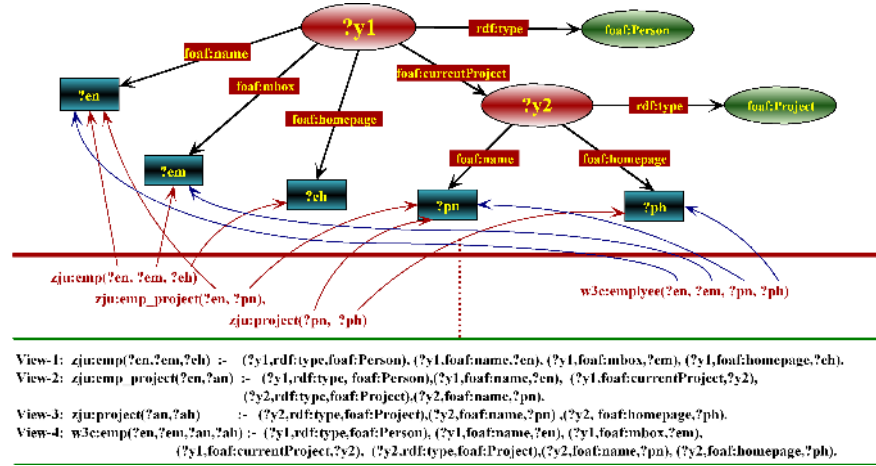
Fig. 3. Mappings from two relational databases with different structures to an ontology. “?en,?em,?eh,?pn,?ph” are variables and represent “employee name”, “employee email”, “employee homepage”, “project name”, “project homepage”, respectively.
