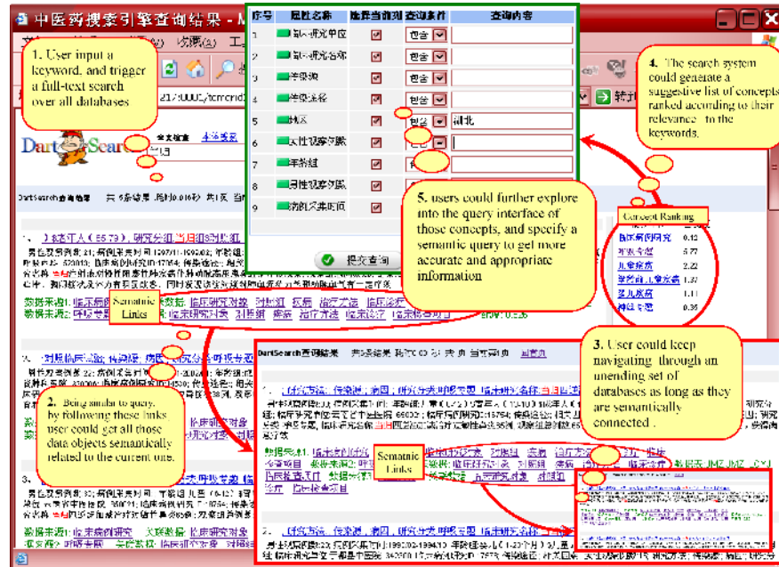
Fig. 7. Intuitive Search Portal with Concept Ranking and Semantic Navigation
