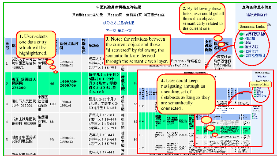
Fig. 6. Semantic navigation through the query results.
