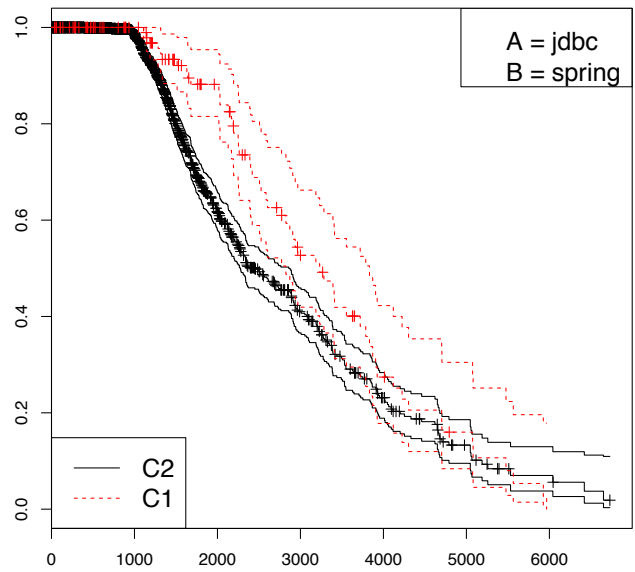
Fig. 3. Survival curves of database framework occurrence in the considered projects.
