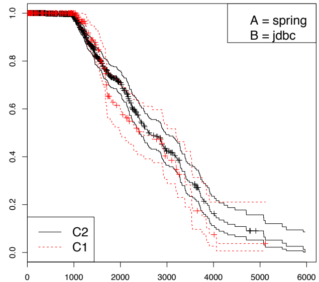
Fig. 4. Survival curves C_1 and C_2 for Spring and JDBC.
