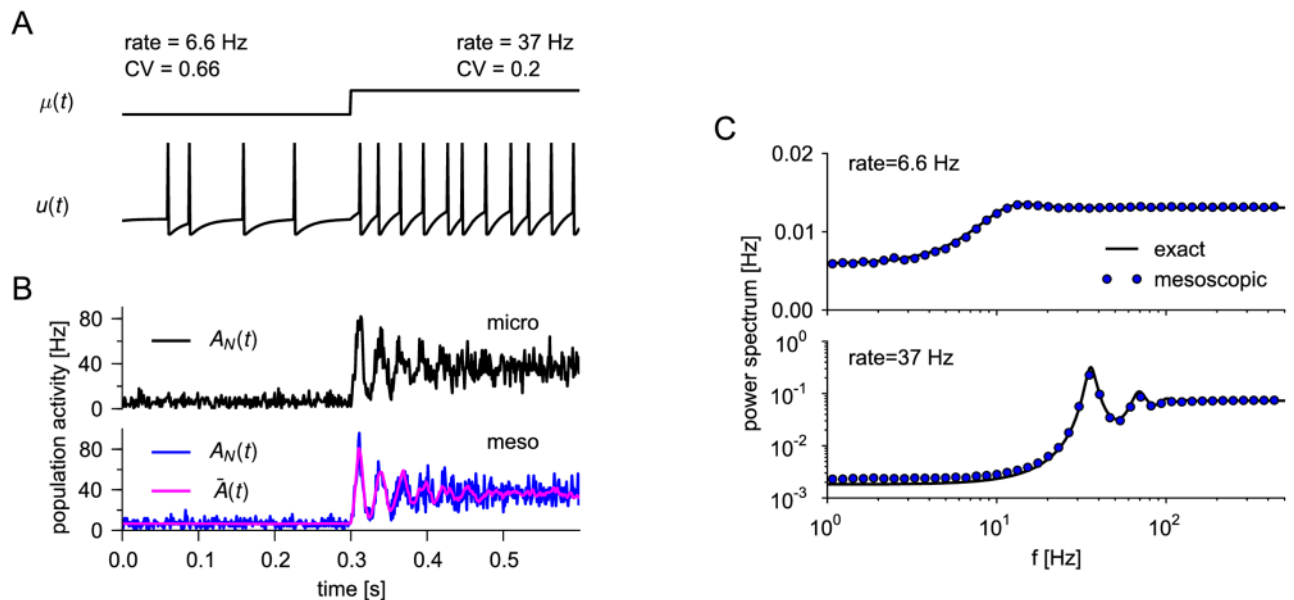
Fig 3. Population activity of uncoupled leaky integrate-and-fire neurons without adaptation. (A) Neurons were stimulated by a step current I_{ext}(t) such that \mu = u_{rest} + RI_{ext}(t) increased from \mu = 15 mV to \mu = 30 mV (top). Voltage trace of one of 500 neurons (bottom). Stationary firing statistics (rate and coefficient of variation (CV) of the interspike intervals) corresponding to the two stimuli are indicated above the step current. (B) Realizations of the population activity A_N(t) for the microscopic (top) and mesoscopic (bottom, blue line) simulation. The magenta line shows the expected population rate \bar{A}(t) given the past actual realization A_N(t) for t' < t . (C) The power spectrum of the stationary activity A_N(t) obtained from renewal theory, Eq (134), (black solid line) and from the mesoscopic simulation (blue circles). The top and bottom panel corresponds to weak ( \mu = 15 mV) and strong ( \mu = 30 mV) constant stimulation (transient removed).
