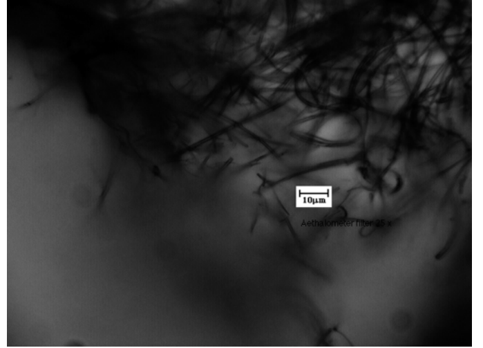
Figure 8. Optical microscope image of the quartz fibers near the surface of pristine aethalometer filter media. The milky appearance is a consequence of multiple scattering by fibers out of the depth of field of the objective. Fibers appear to be randomly oriented, and to have diameters of approximately 1 \mu\text{m} .
