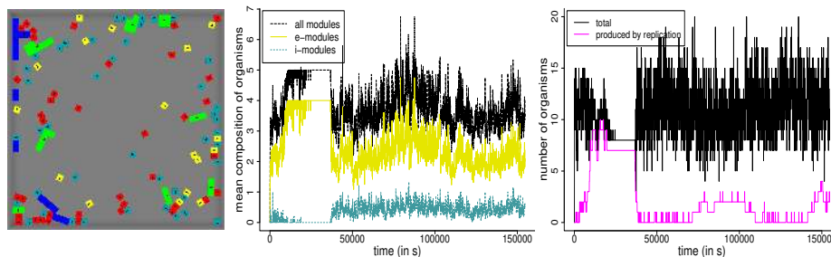
Fig. 2. Left: snapshot taken in a simulation trial (green: organisms, some of which are replicating, blue: polymers without membrane, yellow/turquoise/red: e/i/b -modules). Center: mean composition (i.e., modular makeup) of organisms over time. Right: total number of organisms and number of those produced by replication over time.
