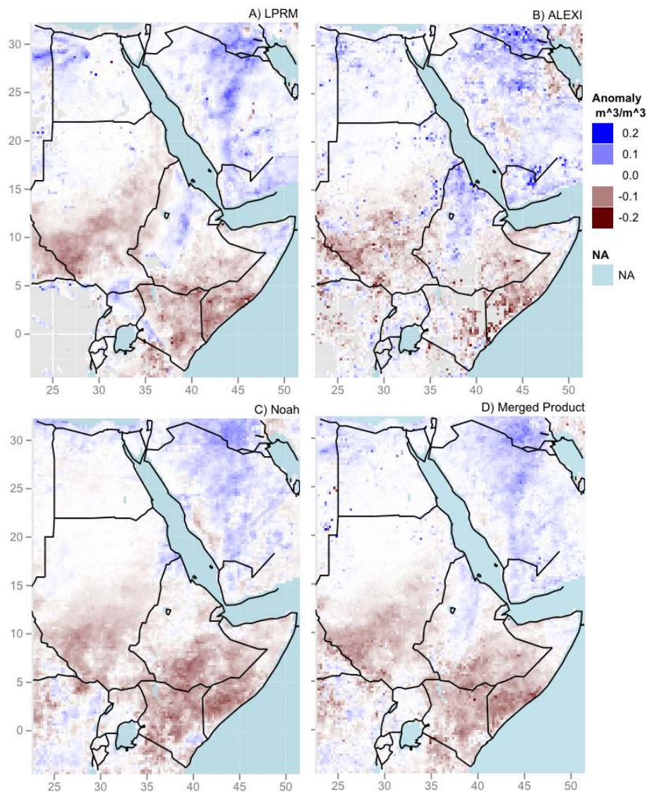
Fig. 10. Individual and merged product anomaly maps for an 8-day period during the 2011 long rainy season (28 April–6 May). (A) LPRM, (B) ALEXI, (C) Noah, (D) Merged product.
