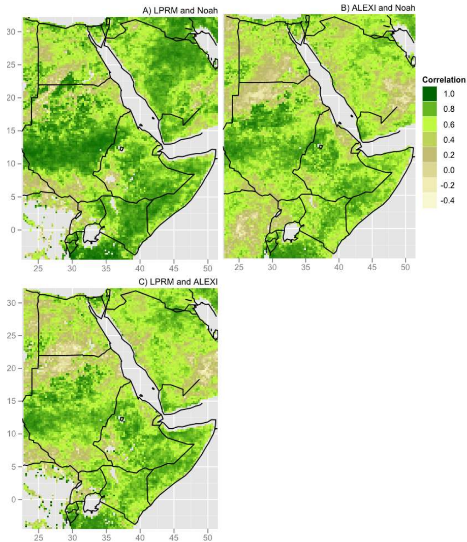
Fig. 5. Temporal cross-correlation of rescaled soil moisture anomalies for January 2007–June 2010 computed between (A) LPRM and Noah, (B) ALEXI and Noah, and (C) ALEXI and LPRM.
