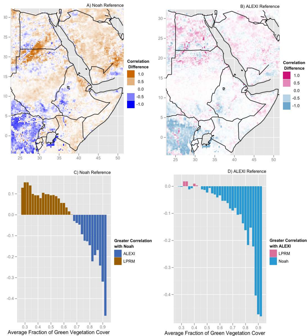
Fig. 6. Anomaly correlation difference using Noah (A, C) and ALEXI (B, D) as reference datasets. Areas shaded in brown or pink represent a greater correlation between LPRM and the reference dataset. (A) and (B) show the spatial distribution of correlation differences, while (C) and (D) show correlation differences as a function of the average fraction of green vegetation during the rainy seasons.
