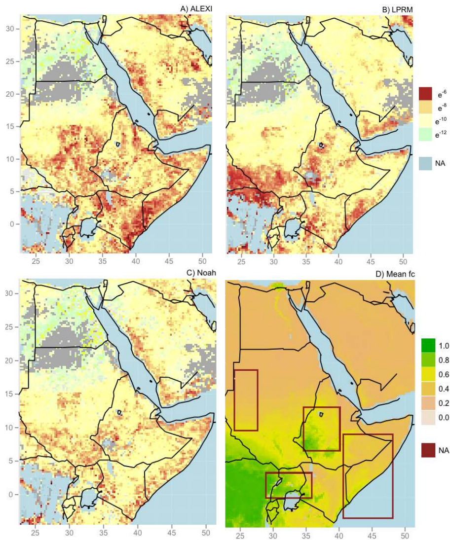
Fig. 7. The variance of the triple collocation analysis-based errors in (\text{m}^3 \text{m}^{-3})^2 for each product juxtaposed with the annual average fraction of green vegetation cover. (A) ALEXI TCA, (B) LPRM TCA, (C) Noah TCA, (D) mean fraction of green vegetation cover over the period 2007 to 2011. Gray areas in panels (A)–(C) indicate regions below the correlation threshold for the TC analysis ( r < 0.2 ). Red boundaries in panel (D) indicate bounding boxes for the analysis in Tables 1–4.
