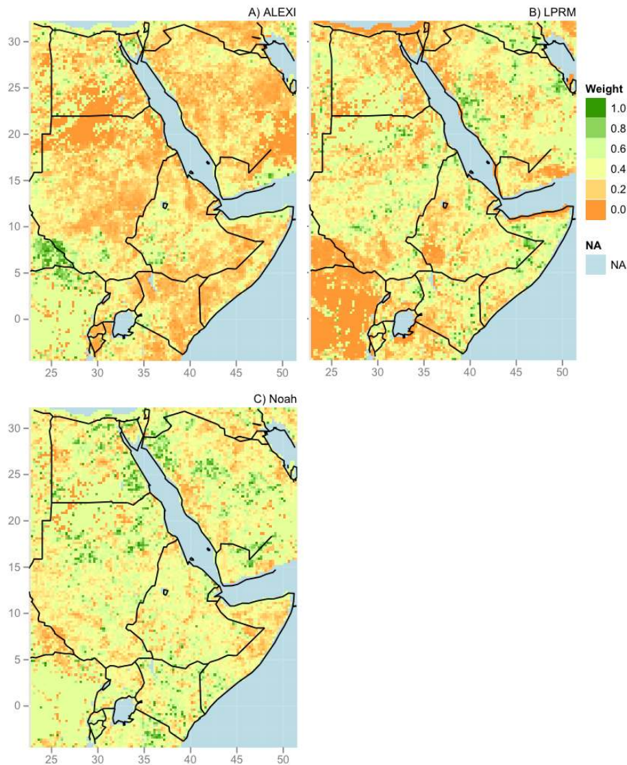
Fig. 9. TCA-based weight map for the case in which data are available from all products for (A) ALEXI, (B) LPRM and (C) Noah. The sum of weights per location adds to unity.
