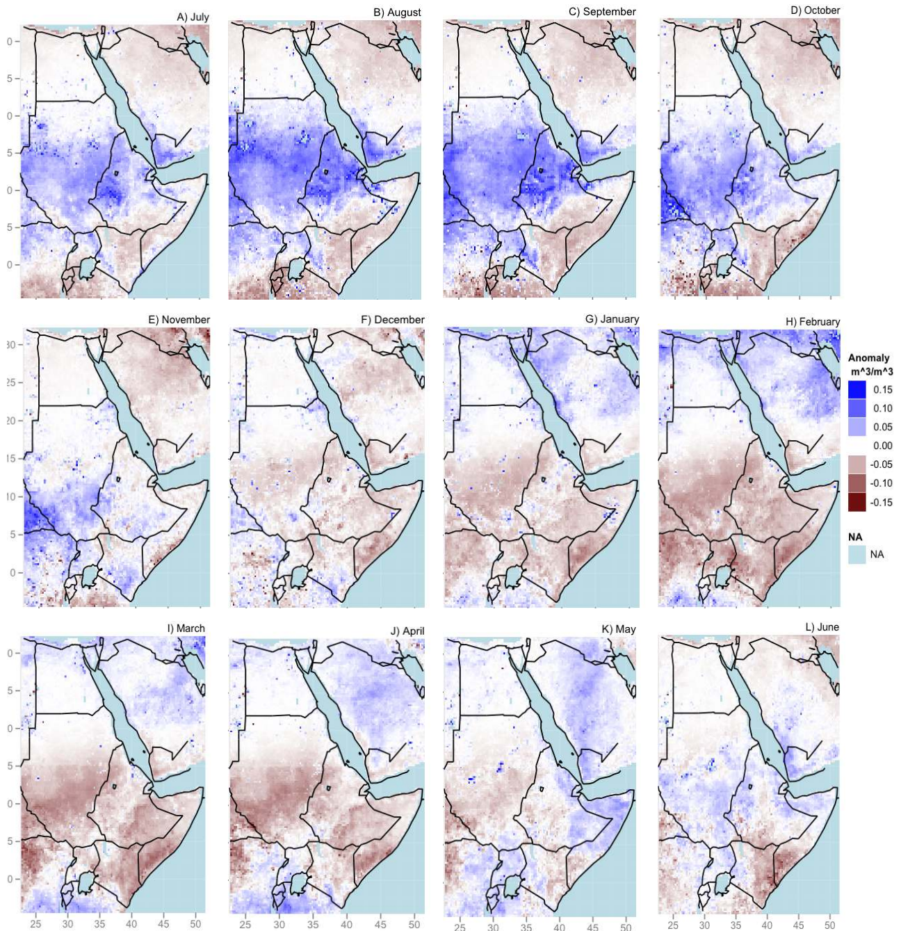
Fig. 11. Monthly anomaly maps of the progression of the 2010–2011 drought using the merged product. July–December 2010 (A–F) and January–June 2011 (G–L).
