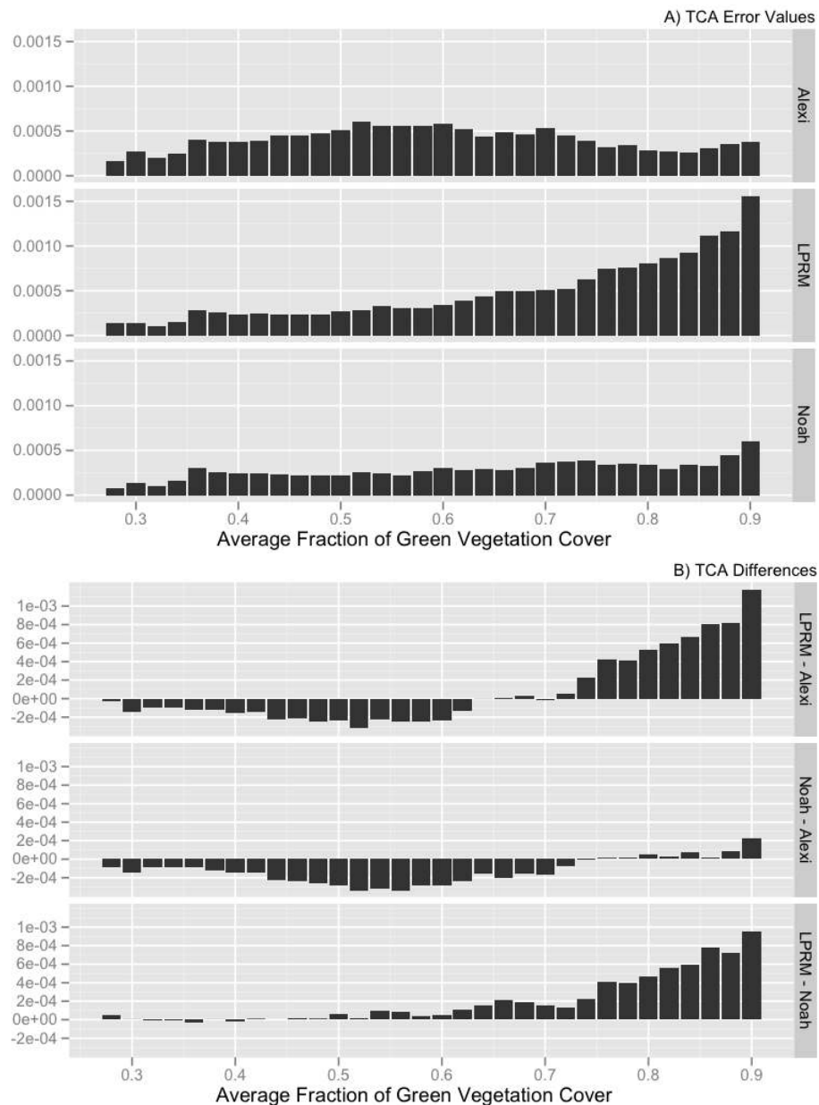
Fig. 8. The variance of the triple collocation analysis-based errors in (\text{m}^3 \text{m}^{-3})^2 binned as a function of average fraction of green vegetation cover during the rainy season, showing (A) TCA error values for each SM retrieval technique, and (B) differences in TCA between retrieval techniques.
