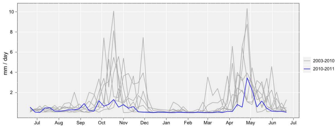
Fig. 2. TMPA 3B42 precipitation estimates from 2003–2011: blue = 2010–2011; gray = all other years.
