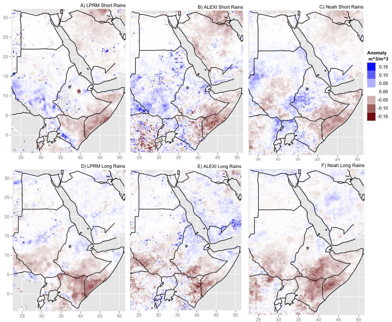
Fig. 4. Seasonal anomalies averaged over the 2010 short rains (A–C) and 2011 long rains (D–F) for LPRM (A, D), ALEXI (B, E) and Noah (C, F). The short rains are defined as the period from 12 September–1 December, while the long rains span 28 March–30 June.
