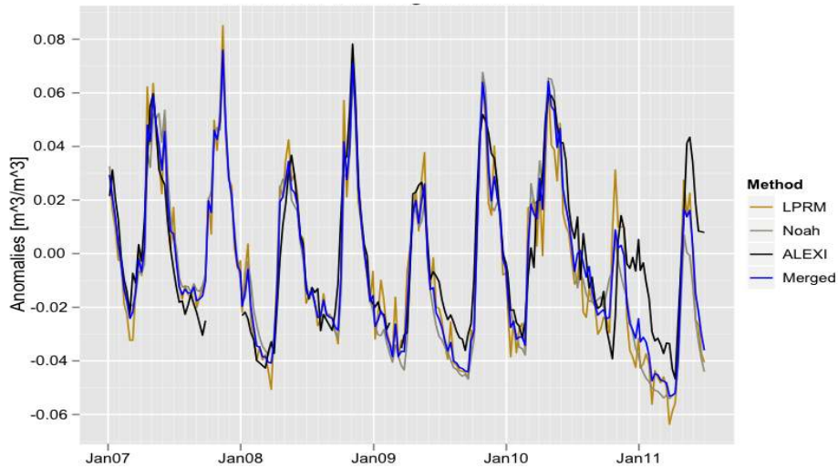
Fig. 12. Comparison of anomalies from individual and merged products using a January 2007–June 2010 baseline, averaged over the area of interest within the Horn of Africa (see Fig. 1).
