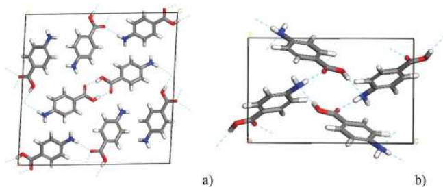
Fig. 2 (a) Unit cell of alpha-PABA with two molecules in the asymmetric unit and eight molecules in the unit cell; packing is comprised of carboxylic acid H-bonding dimers and NH \cdots O H-bonds. (b) Beta-PABA unit cell showing 4-membered H-bonding ring containing NH \cdots O and OH \cdots N interactions.
