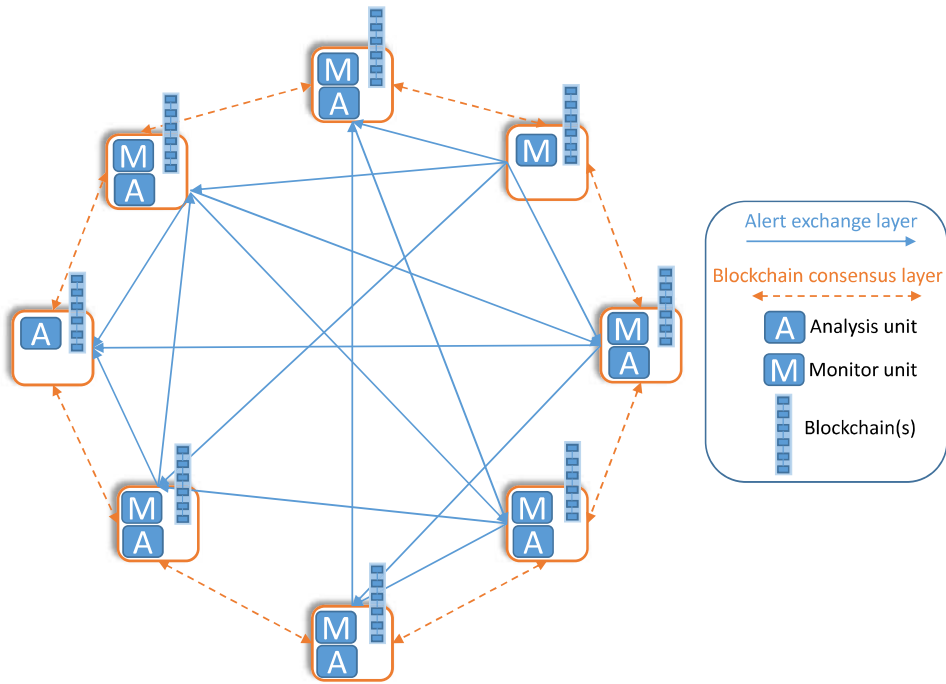
Fig. 1. Generic architecture of a blockchain-based CIDS.
