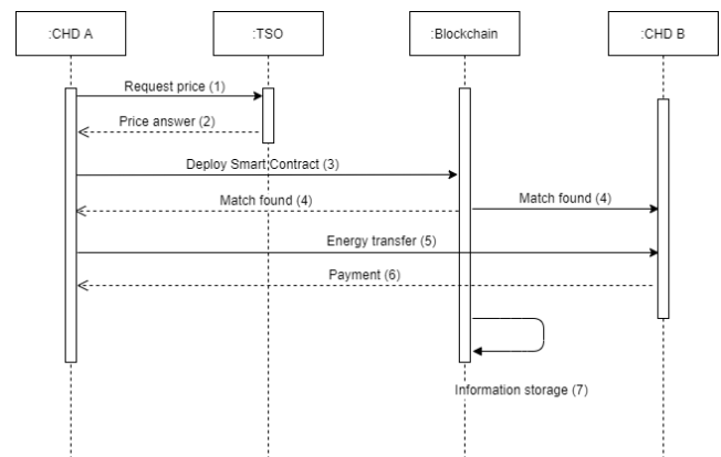
Figure 2. Sequence diagram with the smart contract procedures
