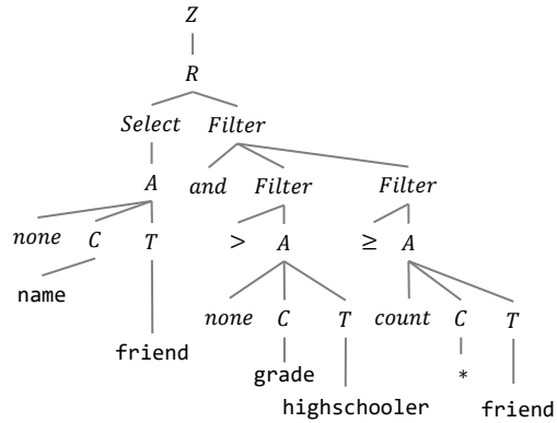
Figure 3: An illustrative example of SemQL. Its corresponding question and SQL query are shown in Figure 1.
