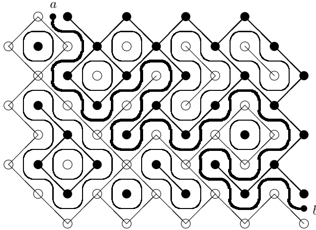
Figure 3. Loop representation of the random cluster model. The sites of the original lattice are colored in black, while the sites of the dual lattice are colored in white. Clusters and dual clusters and loops separating them are pictured. Under Dobrushin boundary conditions besides a number of loops there is an interface running from a to b , which is drawn in bold. Weight of the configuration is proportional to (\sqrt{q})^{\# \text{ loops}} .
