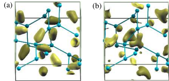
FIG. 4 (color online). (a) and (b) show the partial charge density of the VBM and CBM states at (0.17, 0.17, 0.17) for \text{Si}_{20}\text{-T} , respectively. It can be seen that the states distribute mostly around the Si triangles.
