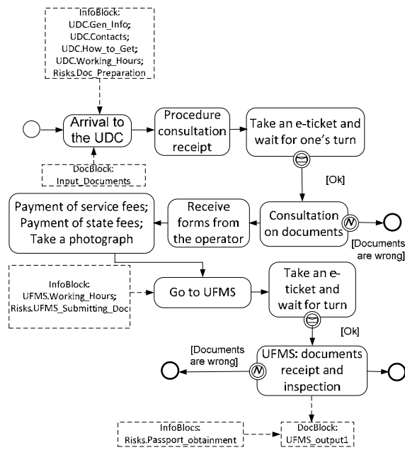
Figure 4: A process model example
