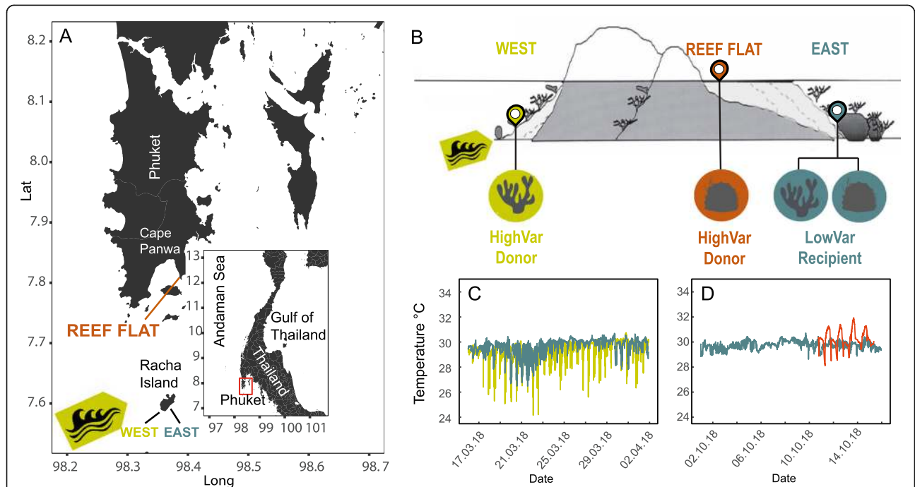
Fig. 2 Collection sites and environmental properties. a Coral sites at Racha Island and Panwa reef flat in the Andaman Sea south of Phuket Island in Thailand (red rectangle). The impact of large-amplitude internal waves creates high variability habitats on the western shore of Racha Island (light green arrow). At the shallow reef flat in Panwa, high variability and extreme conditions are linked to diurnal solar and tidal variation. b Three distinct reef sites were selected: a high variability west shore site of Racha Island (“HighVar,” 15 m depth, light green); a high variability reef flat in Phuket Island, Panwa (“HighVar,” 0–2 m depth, orange); and a sheltered low variability reef site of stable environmental conditions at Racha Island east shore (“LowVar,” 15 m, teal). Corals from “HighVar” environments were designated as microbiome donors, whereas corals from the “LowVar” site were used as recipients during microbiome transplantation experiments. c, d In situ temperature profiles show the temperature history of corals prior to experiments. Strong fluctuations of temperature were measured at the “HighVar” west shore site (light green in c ) and reef flat (orange in d ), while comparably stable conditions are shown for the “LowVar” east shore site (teal in c and d ). Branching coral, Pocillopora sp.; massive coral, Porites sp.
