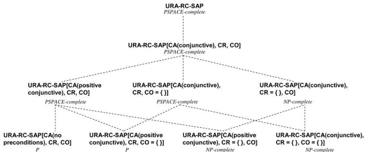
Fig. 3. Summary of computational complexity results for various cases of URA\text{-}RC\text{-}SAP . A dotted line links a case to a subcase. For example, URA\text{-}RC\text{-}SAP[CA(\text{positive conjunctive}), CR, CO] is a subcase of URA\text{-}RC\text{-}SAP[CA(\text{conjunctive}), CR, CO] .
