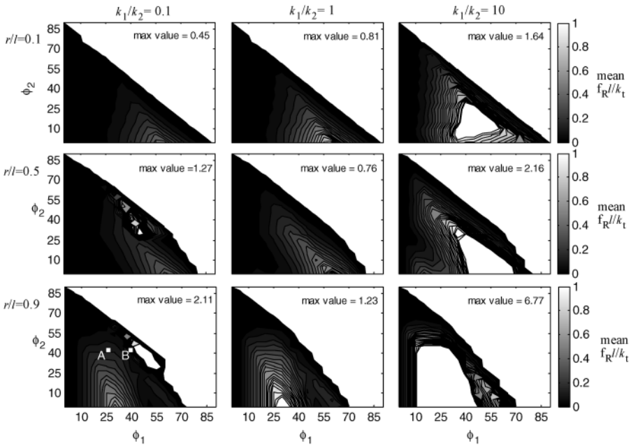
Figure 6. Average normalized force ( \bar{f}_{Rl}/k_T ) for link length normalization. Contours are in increments of 0.05 up to 1.00. The joint rest angles \varphi_1 and \varphi_2 are in degrees. Darker colors (lower contours) represent lower forces and thus better parameter configurations.
