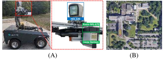
Fig. 7: Experimental setup for FR-IOSB data set.
