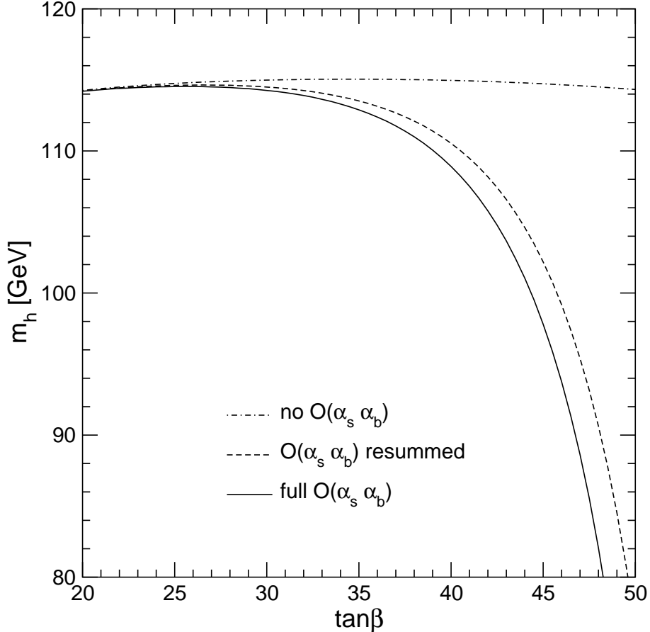
Figure 2: The result for the lightest \mathcal{CP} -even Higgs-boson mass in the MSSM, m_h , as obtained with the program FeynHiggs is shown as a function of \tan\beta for M_A = 120 GeV, \mu = -1 TeV, M_{\tilde{t}_L} = M_{\tilde{t}_R} = M_{\tilde{b}_R} = m_{\tilde{g}} = 1 TeV, A_t = A_b = 2 TeV. The meaning of the different curves is explained in the text.
