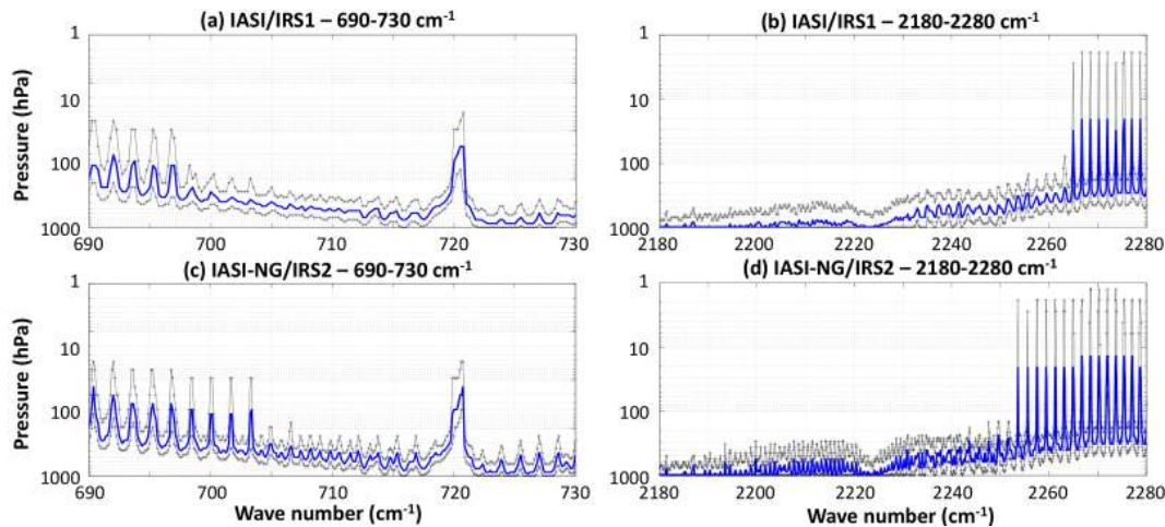
Figure 4. Pressure of the maximum (blue line) and of the half-height width (black) of the temperature Jacobians at the IASI spectral resolution in the 15 \mu\text{m} (a) and 4.3 \mu\text{m} (b) bands and at the IASI-NG spectral resolution in the 15 \mu\text{m} (c) and 4.3 \mu\text{m} (d) bands. The Jacobians have been computed by 4A and averaged over the whole tropical atmospheric situations of the TIGR database.
