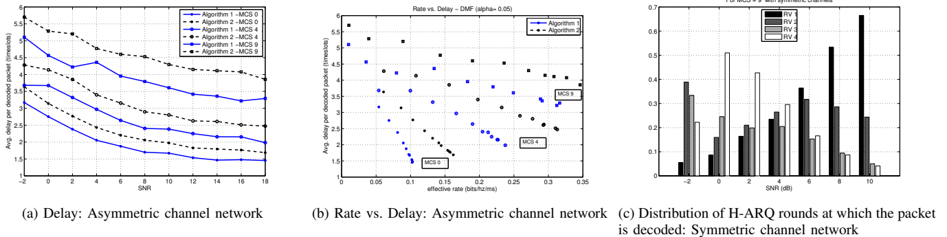
Fig. 5: Various performance comparisons of two algorithms with DMF relaying
