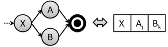
Figure 11: Workflow with corresponding Genome
