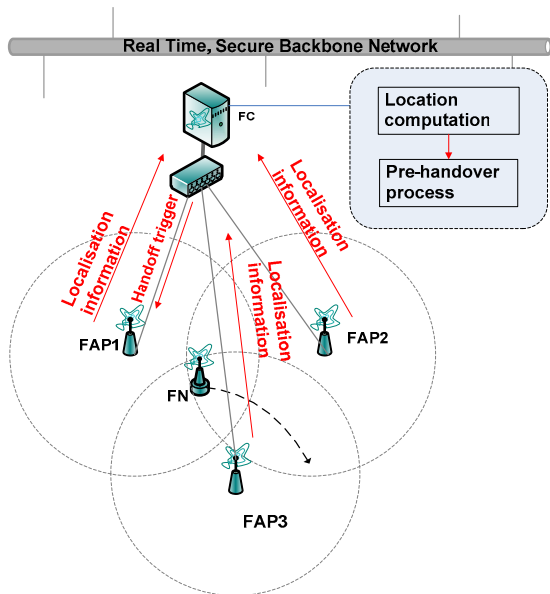
Figure 3. Handover concept in FlexWare.
