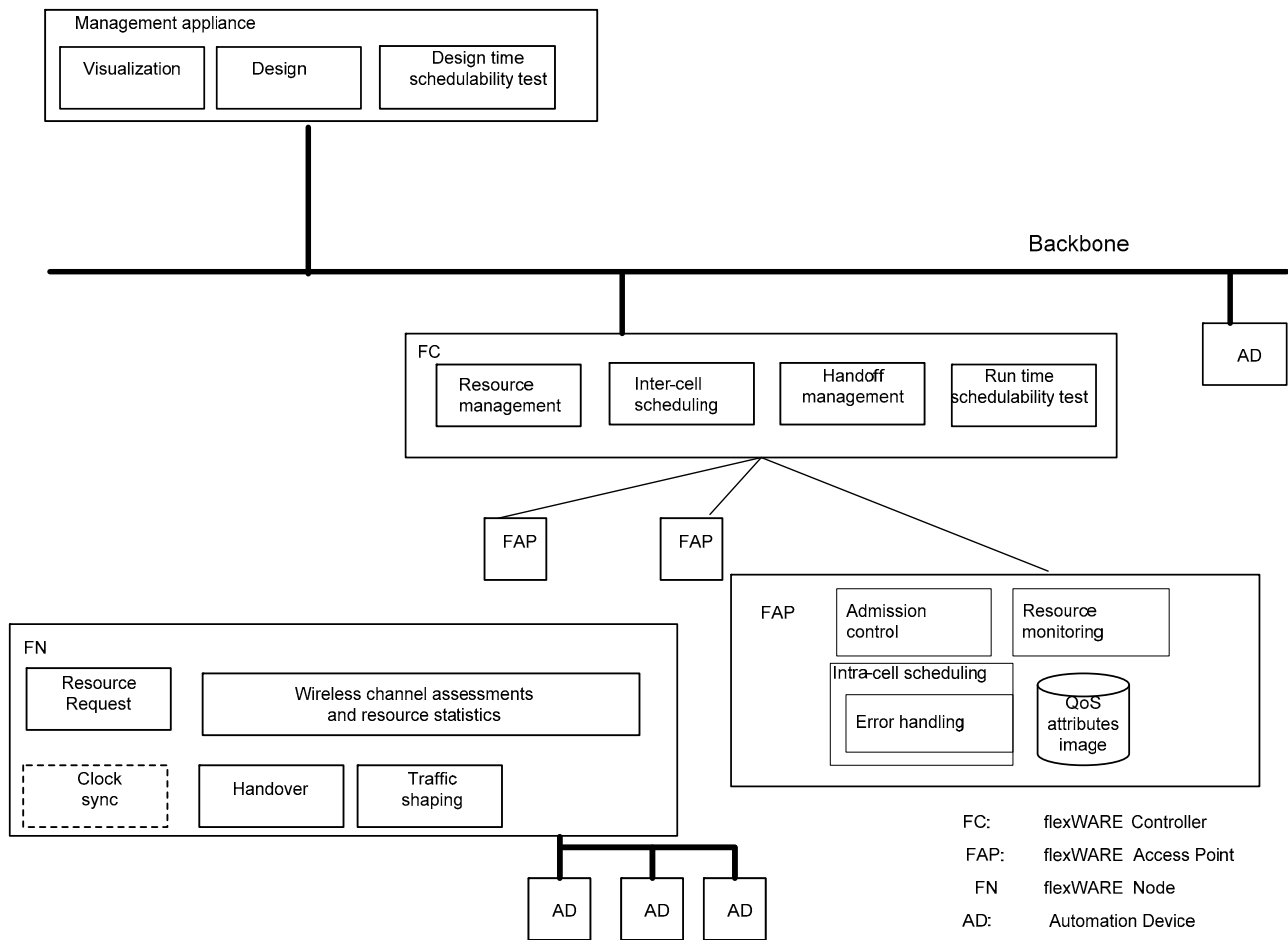
Figure 3. The FlexWare QoS architecture.
