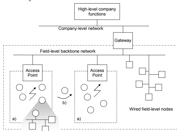
Figure 1. Two-level hierarchy of a hybrid wired/wireless factory automation network.
