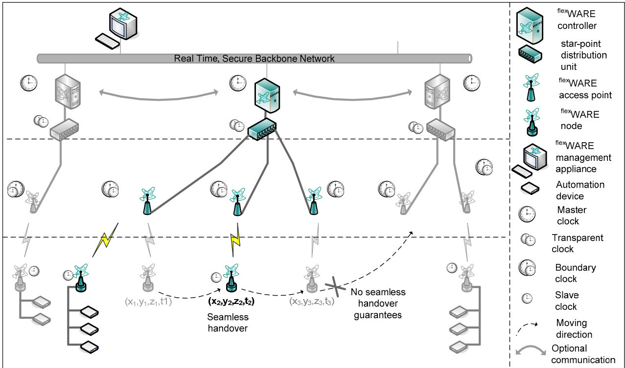
Figure 2. FlexWare system architecture.
