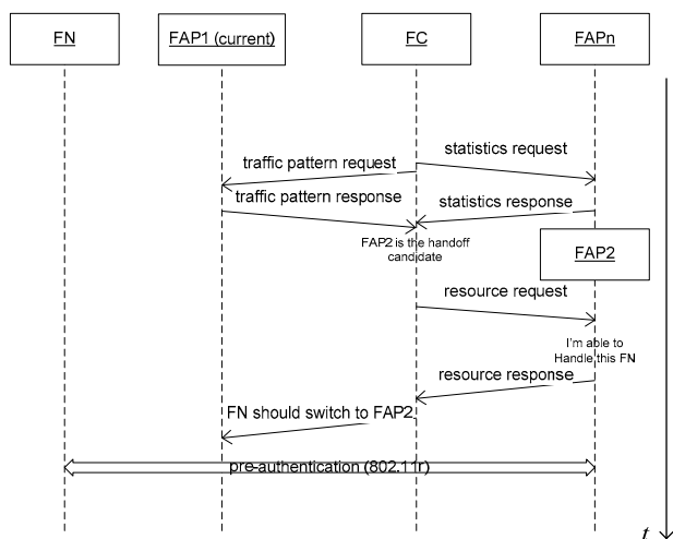
Figure 4. Sequence of messages in the handover procedure.
