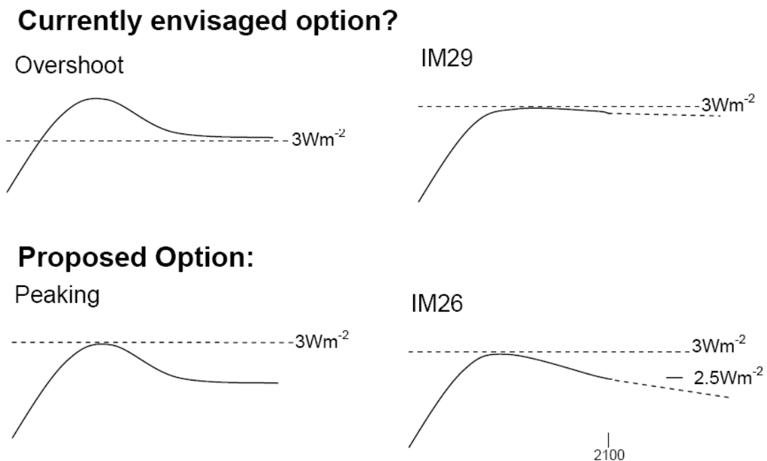
Figure 2 - Schematic illustration of peaking and overshooting pathways and the envisaged IM29 and IM26 options. Note that IM29 would neither allow studying effects to decreasing forcing, nor cover the lower forcing levels beyond 2050 representative for the emission categories I and II. In regard to the radiative forcing trajectories of the IM scenarios, compare figure III.2 (right) in the Background note to participants and Figure 3 below.
