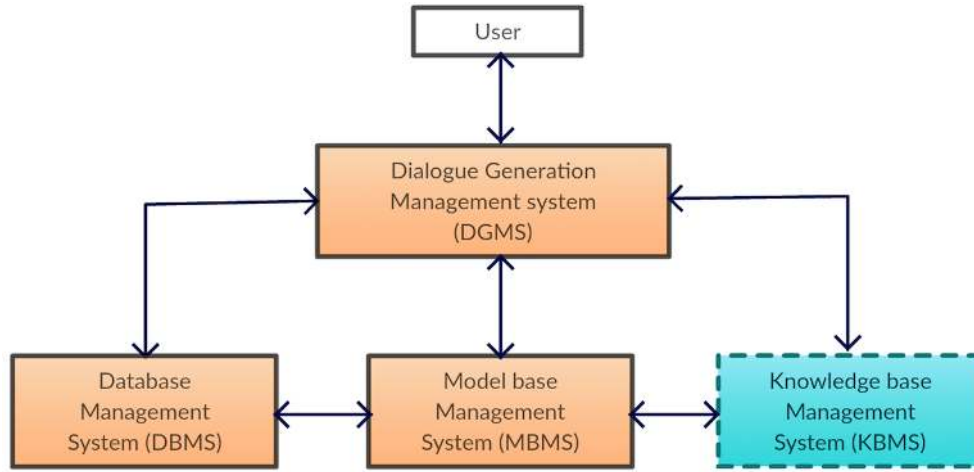
Figure 2: The basic components of an intelligent and knowledge-based DSS.
