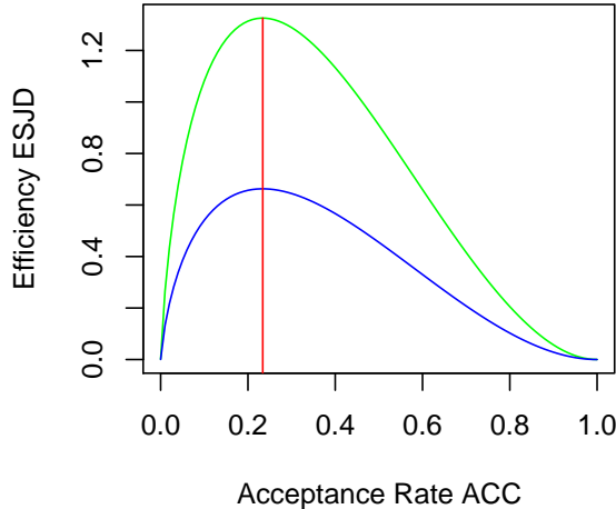
Figure 7: A graph of the relationship between the expected squared jumping distance (ESJD) and asymptotic acceptance rate (ACC), as described in equations (16) (top, green) and (8) (bottom, blue), in units where dI(\beta) = 1 .
