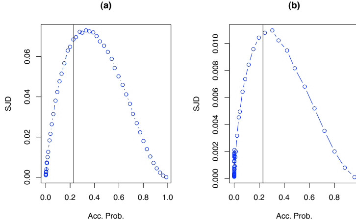
Figure 4: SJD versus Acceptance Probability for the inhomogeneous Gaussian case f_i = N(0, i^2) and f_i^\beta = N(0, i^2\beta^{-1}) , in dimensions (a) d = 10 and (b) d = 100 .
