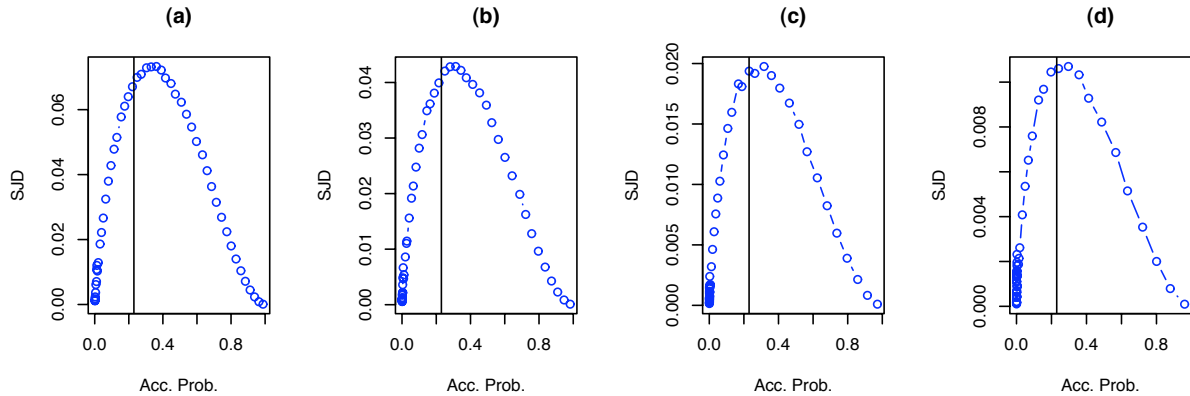
Figure 3: squared jump distance (SJD) versus estimated Acceptance Probability for the Gaussian case f = N(0, 1) and f^\beta = N(0, \beta^{-1}) , in dimensions (a) d = 10 , (b) d = 20 , (c) d = 50 , and (d) d = 100 .
