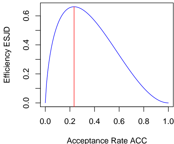
Figure 2: A graph of the relationship between the expected squared jumping distance (ESJD) and asymptotic acceptance rate (ACC),
