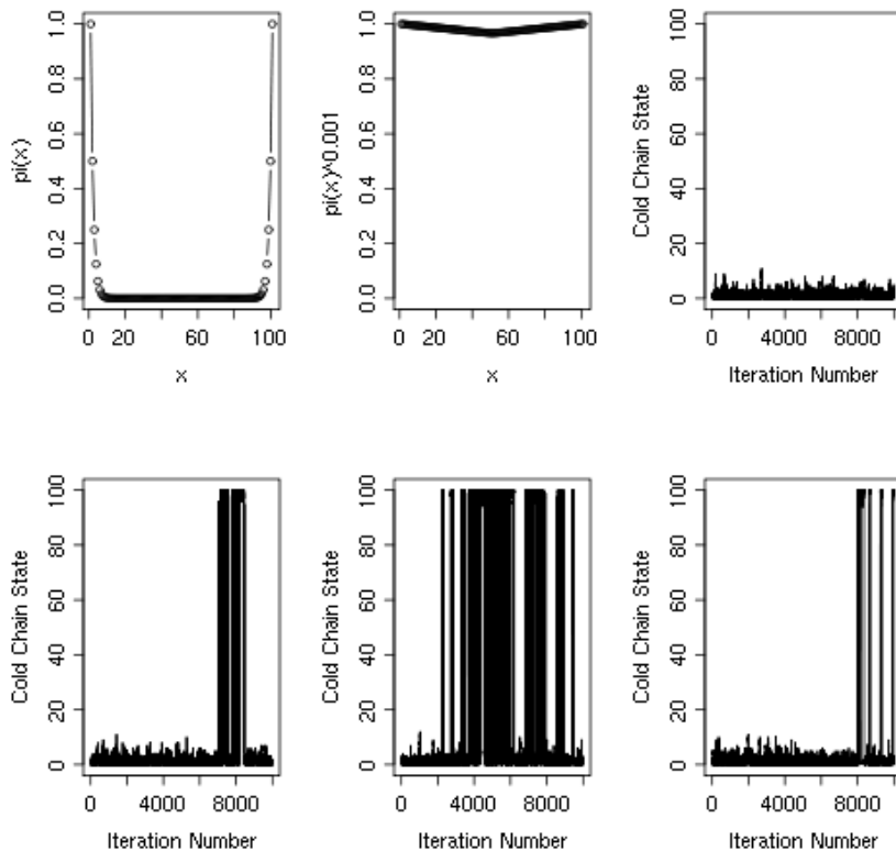
Figure 1: The toy example’s target density (top-left), tempered density at inverse-temperature \beta = 0.001 (top-middle), random-walk Metropolis run (top-right), and trace plots of the cold chain over 10,000 full iterations of
