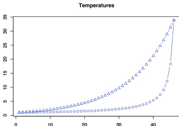
Figure 5: The temperatures \{T_j\} selected for the Ising model (triangle: geometric spacing; circle: 23% rule).
