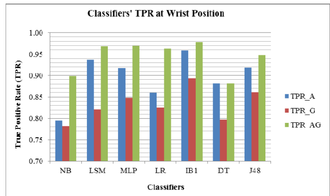
Fig. 3. Overall TPR results: it almost follows the same pattern as in Fig. 1 and Fig. 2 except that the improvement done by the combination of the two sensors, gets relatively better compared to their individual TPR.
