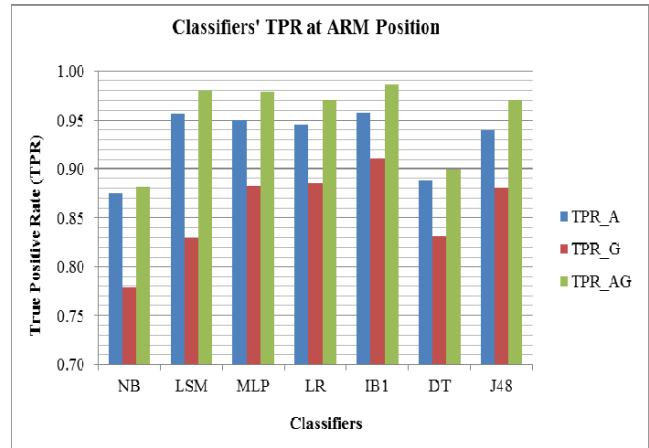
Fig. 1. Overall TPR results for an accelerometer (A), a gyroscope(G) and their combination (AG): Overall, an accelerometer performs better than a gyroscope. However, when both are used in combination, the results are further improved than their individual results.
