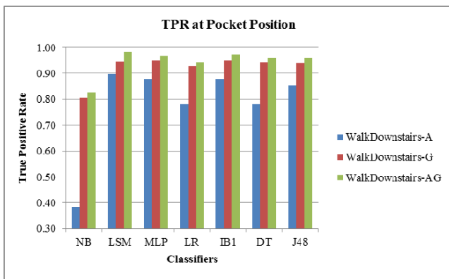
Fig. 5. The walking downstairs activity is better recognized by the combination of an accelerometer and a gyroscope compared to their individual recognition. Moreover, the gyroscope performs better than the accelerometer here.
