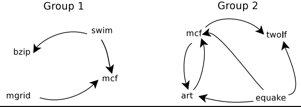
Figure 13. Contention relations of two groups of SPEC-CPU2000 benchmarks. If A points to B, that means B has more than 50% performance degradation when running together with A on a shared cache, compared to running alone when B can monopolize the whole cache.
