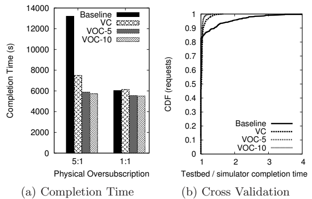
(a) Completion Time (b) Cross Validation Figure 16: Testbed experiments show that virtual networks provide performance gains and validate our simulator.
