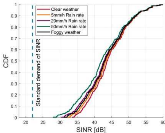
Figure 8. SINR distribution for different wheather conditions for Hanover network described in [6]
