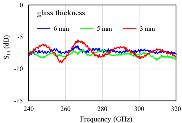
Figure 5. Measurement results of reflection characteristics of different types of glasses
