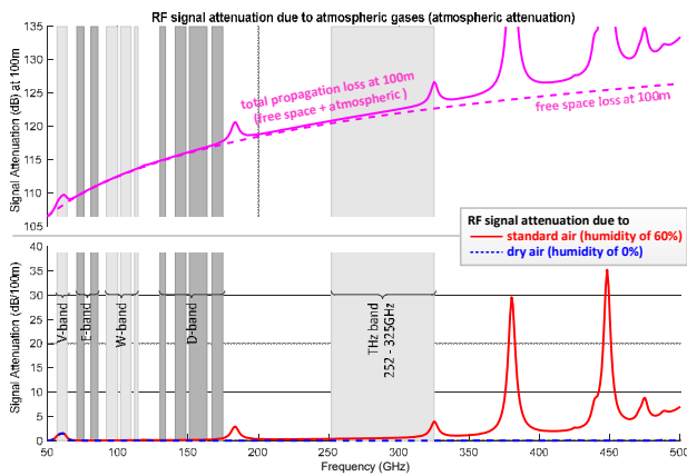
Figure 2. Frequency-dependent RF signal attenuation due to atmospheric gases (atmospheric attenuation), and as a reference, total propagation loss (free space loss + atmospheric attenuation) at a distance of 100 m.
