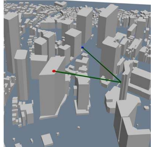
Figure 3. Example for connecting two antennas without LOS in the Shinjuku area via one reflection
