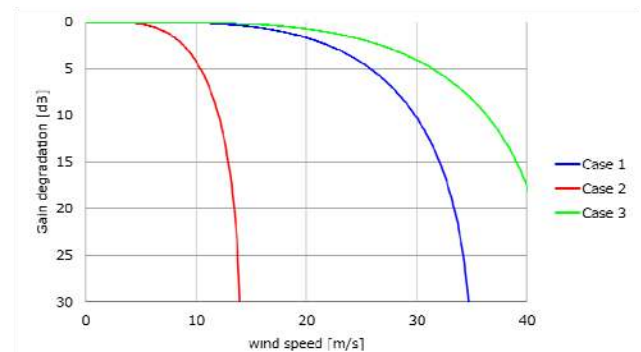
Figure 6: Wind speed vs. Gain degradation for three cases of pole thickness and pole height
