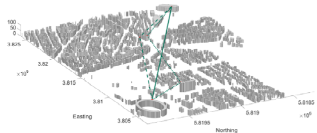
Figure 1. Exemplary simulation scenario at Berlin with links connecting the Olympic Stadium with the International Congress Center
