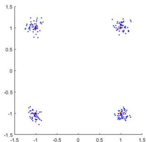
Figure 7. Signal vector configuration from link level simulation of the propagation scenario shown in Figure 2.
