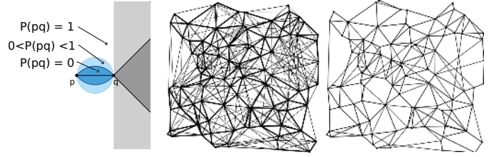
Fig. 7. Stochastic empty region graphs. Left: Edge pq exists with probability P = 1 if no point exists within the light blue region; with probability P < 1 if at least one point exists within the light blue region; and with probability P = 0 if at least one point exists within the dark blue region. Middle: sERG encoding probability. Thick edges have a larger probability than thin edges. Right: A random draw of this sERG.
