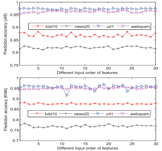
Fig. 7. Prediction accuracies on varied input orders of features (the top figure with J48 while the bottom figure with KNN)
