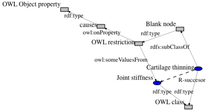
Fig. 1. RDF graph corresponding to causal chain encoding OWL axiom
