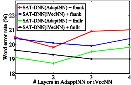
Figure 2: Performance of SAT-DNN as the number of layers in AdaptNN and iVecNN increases. WER(%) is measured on the HUB’00-SWB set.
