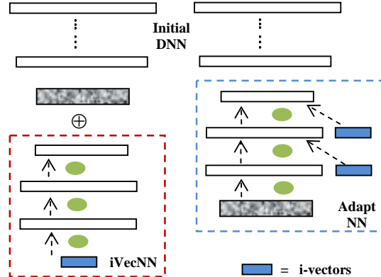
Figure 1: Illustration of the iVecNN and AdaptNN methods for input feature mapping. The green circles mark the connection parameters for the feature mapping networks.
