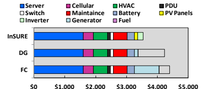
Figure 22: Annual depreciation cost
