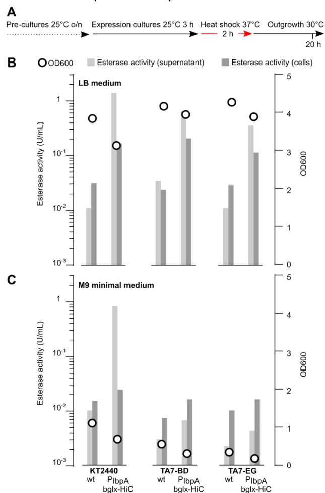
Figure 8: Comparing P_{lbpA} -PET hydrolase expression in LB versus M9 minimal medium. (A) Experimental protocol to test genomically integrated P_{lbpA} -bglx-HiC construct expression in different culture media. (B) OD600 and esterase activities of cultures in LB medium including P. putida KT2440, TA7-EG, and TA7-BD, either as the non-hydrolase expressing strains (labelled wt) or with the genomically integrated P_{lbpA} -bglx-HiC cassette. (C) OD600 and esterase activities of P. putida KT2440, TA7-EG, and TA7-BD, either as the wt strains or with the genomically integrated P_{lbpA} -bglx-HiC cassette, in M9 minimal medium with 20 mM citrate (KT2440), 10 mM TA + 10 mM BD (TA7-BD) or 10 mM TA + 10 mM EG (TA7-EG). Data depict one representative experiment with duplicate cultures.
