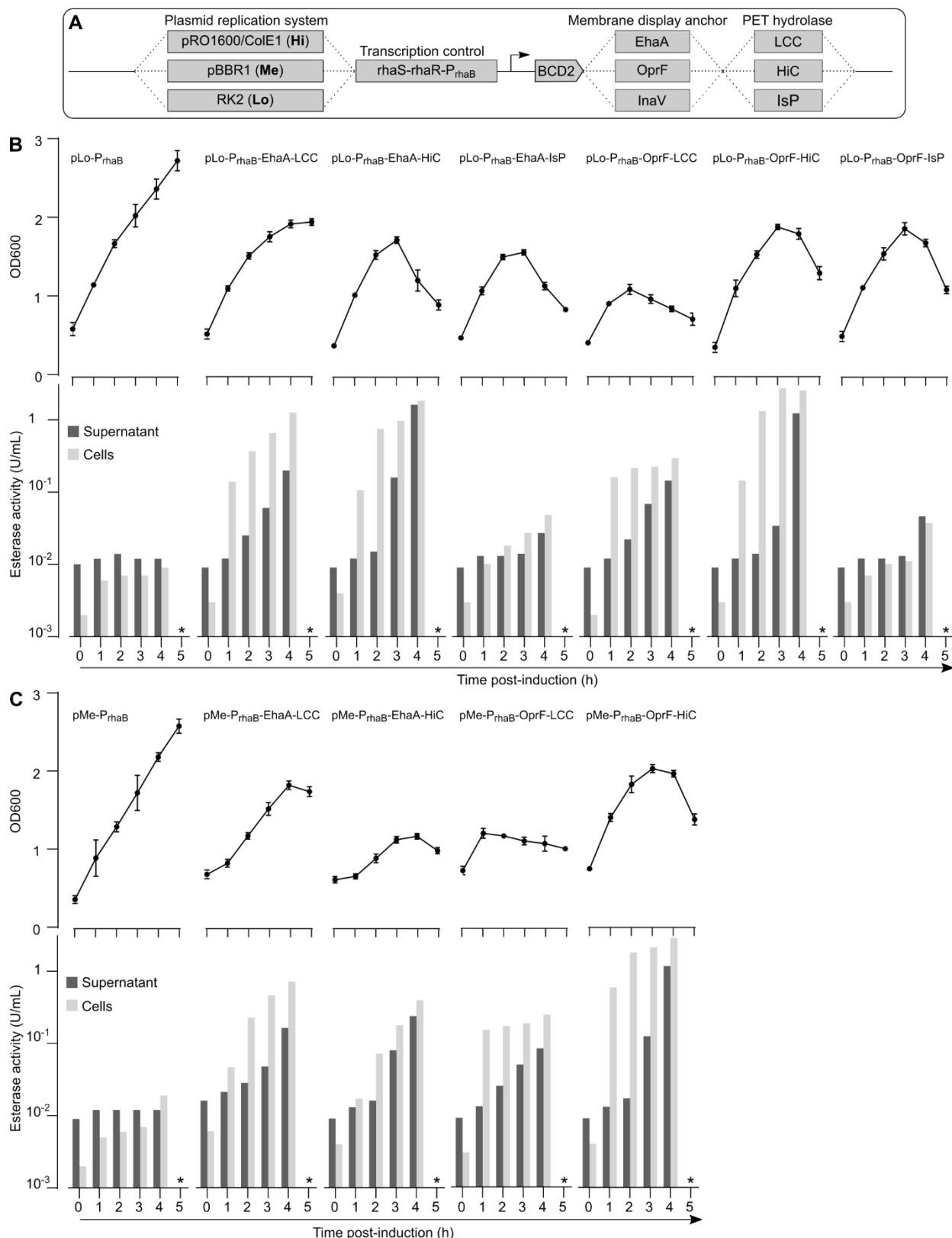
Figure 3: Testing PET hydrolase membrane display systems. (A) Overview of combinatorial test construct design for PET hydrolase membrane expression, including plasmids providing low, medium, and high cellular copy number, transcriptional control by the P_{rhaB} system, translation initiation via the BCD2 translational coupler, three different membrane display anchors, and three different PET hydrolases. (B) OD600 and esterase activity of P. putida TA7-EG shake flask cultures expressing the indicated display constructs from the RK2 low copy number plasmid, measured for 5 h post-induction (induction at t=0 h). (C) OD600 and esterase activity of P. putida TA7-EG shake flask cultures expressing the indicated display constructs from the pBBR1 medium copy number plasmid, measured for 5 h post-induction (induction at t=0 h). The * in (B) and (C) indicates that esterase activity was not measured at the t=5 h timepoint due to obvious cell lysis. Data shown are derived from one representative experiment with duplicate cultures.
