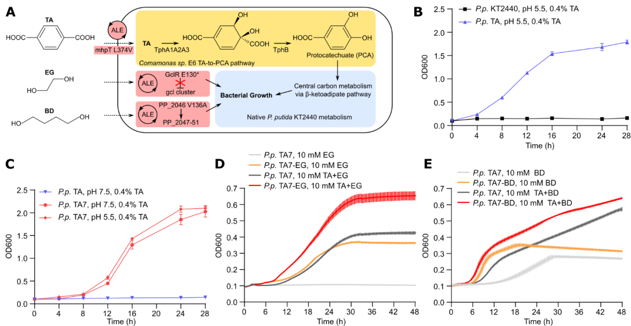
Figure 2: Engineering TA, EG and BD metabolism in P. putida . (A) Overview of the engineering steps, including genomic insertion (yellow) and ALE (red), to endow P. putida with the capacity to use TA, EG and BD as sole carbon sources. (B) Growth of P. putida KT2440 and P. putida TA in shake flasks with M9 minimal medium, 0.4% TA, pH 5.5. (C) Growth of P. putida TA and P. putida TA7 in shake flasks with M9 minimal medium, 0.4% TA, pH 5.5 or pH 7.5. (D) Growth of P. putida TA7 and P. putida TA7-EG analyzed in a plate reader assay with M9 minimal medium, 10 mM EG or 10 mM EG + 10 mM TA, pH 7.5. (E) Growth of P. putida TA7 and P. putida TA7-BD analyzed in a plate reader assay with M9 minimal medium, 10 mM BD or 10 mM BD + 10 mM TA, pH 7.5. Data shown are mean and SD, n=2 (B and C) or n=6 (D and E).
