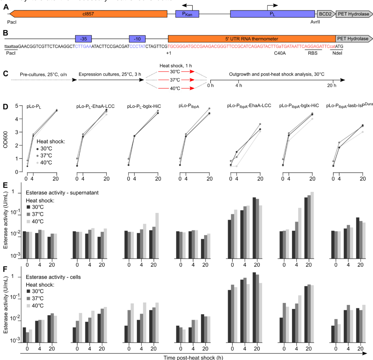
Figure 5: Testing P L and P lbpA heat shock inducible promoters. (A) Overview of the cl857/P L system; this transcriptional regulatory unit spans 1410 bp from the PaclI to the AvrII site. (B) Sequence overview and relevant features of the P lbpA system used here. (C) Experimental protocol to test PET hydrolase expression from P L and P lbpA upon heat shock. (D) OD600 of cultures expressing PET hydrolases in dependence on the heat shock regime. (E) Esterase activity of cultures expressing PET hydrolases in dependence on the heat shock regime; top, esterase activity in the supernatant; bottom, cell-associated esterase activity. Data shown are derived from one representative experiment with duplicate cultures.
