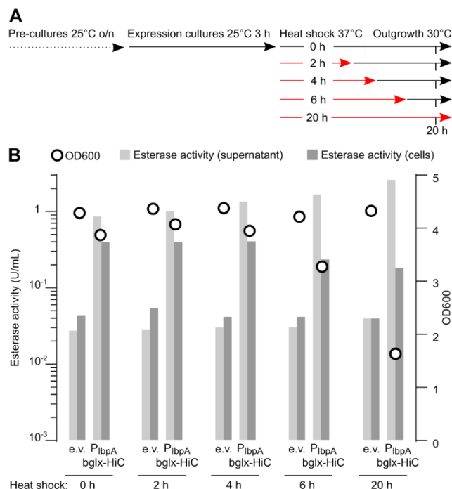
Figure 6: Defining P_{IbpA} temperature-dependent expression output. (A) Experimental protocol to test PET hydrolase expression from P_{IbpA} upon different heat shock regimes. (B) OD600 and esterase activities of P. putida TA7-EG cultures transformed with pLo- P_{IbpA} (empty vector, e.v.), or pLo- P_{IbpA} -bglx-HiC in dependence on the heat shock regime. Data shown are derived from one representative experiment with duplicate cultures.
