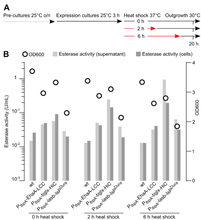
Figure 7: Testing expression of P. putida KT2440 P_{lbpA} -PET hydrolase knock-in strains. (A) Experimental protocol to test the expression of genomically integrated P_{lbpA} -PET hydrolase constructs upon different heat shock regimes. (B) OD600 and esterase activities of P. putida KT2440 (wt) or the corresponding P_{lbpA} -EhaA-LCC, P_{lbpA} -bglx-HiC, and P_{lbpA} -lasb-ISP Dura knock-in strains in dependence on the heat shock regime. Data depict one representative experiment with duplicate cultures.
