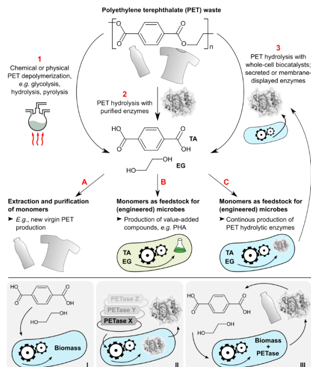
Figure 1: Synthetic PETtroph in relation to other biocatalytic strategies for PET waste valorization. Top panel: PET waste can be depolymerized to TA and EG using chemical means (1), with purified PET hydrolases (2), or using whole-cell biocatalysts displaying or secreting PET hydrolases (3). TA and EG can be extracted and processed into new virgin PET (A); used as feedstocks for engineered microbes and production of value-added bioproducts (B); or used as feedstocks for engineered microbes producing PET hydrolases in a CBP-like one-pot system (C). Path 2-A was explored by Tournier et al. 19 and Lu et al. 20 ; path 1-B was explored by Kenny et al. 22,33 , Werner et al. 34 and Kim et al. 25 ; path 2-B was described by Tiso et al. 24 and Lu et al. 20 ; path 3-C is what I. sakaiensis performs natively 26 and was explored in this study. Additionally, several recent studies described whole-cell biocatalysts displaying or secreting PET hydrolases (3) without attempting downstream extraction or microbial utilization of released monomers. Bottom panel: sequence of engineering steps attempted in this study. First, we installed TA, EG or BD metabolism in P. putida using genetic engineering and adaptive laboratory
