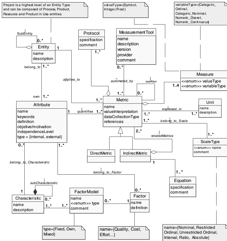
Fig. 2. Conceptual model for the domain of metrics.
