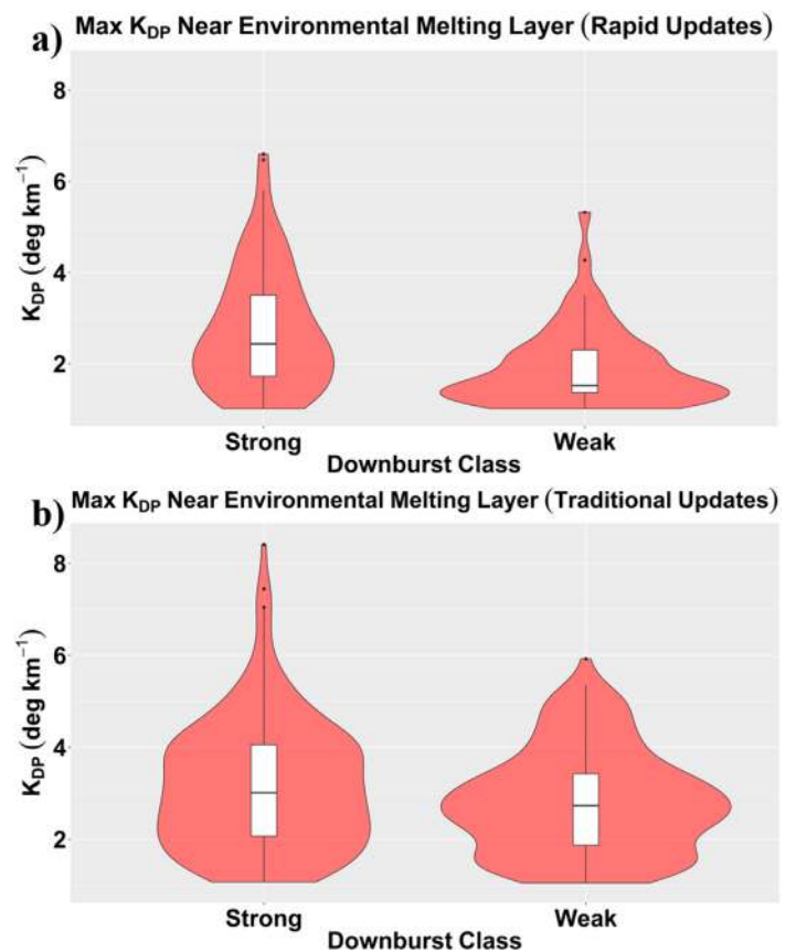
Fig. 5. Violin plots showing the maximum K_{DP} values within the K_{DP} core at the elevation angle closest to the environmental melting layer for (a) rapid-update ( \sim 2 -min) KOUN data and (b) traditional update ( \sim 5 – 6 -min) WSR-88D data. Strong downbursts had a maximum radial velocity of 19.5 \text{ m s}^{-1} or higher, while weak downbursts had a maximum radial velocity of less than 19.5 \text{ m s}^{-1} . The red area of the plot shows the probability density with a greater width indicating a higher frequency of occurrence. Associated boxplots are included within each violin plot for reference.
