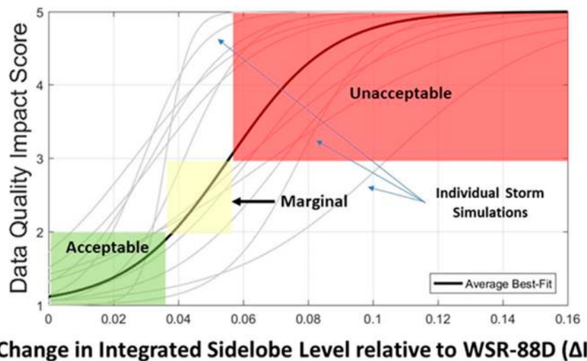
Fig. 11. Fitted data quality impact score vs \Delta\text{ISL} for each of 12 storm cases, and the average best-fit curve (dark line). The x axis is \Delta\text{ISL} in linear units, defined as the difference between the ISL of the radar under test and the ISL of the WSR-88D. \Delta\text{ISL} increases with larger (less acceptable) sidelobe levels.
