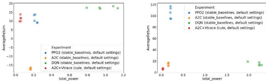
Figure 5: We evaluate A2C, PPO, DQN, and A2C+VTraces on PongNoFrameskip-v4 (left) and BreakoutNoFrameskip-v4 (right), two common evaluation environments included in OpenAI Gym. We train for only 5M timesteps, less than prior work, to encourage energy efficiency and evaluate for 25 episodes every 250k timesteps. We show the Average Return across all evaluations throughout training (giving some measure of both ability and speed of convergence of an algorithm) as compared to the total energy in kWh. Weighted rankings of Average Return per kWh place A2C+Vtrace first on Pong and PPO first on Breakout. Using PPO versus DQN can yield significant energy savings, while retaining performance on both environments (in the 5M samples regime). See Appendix F for more details and results in terms of asymptotic performance.
