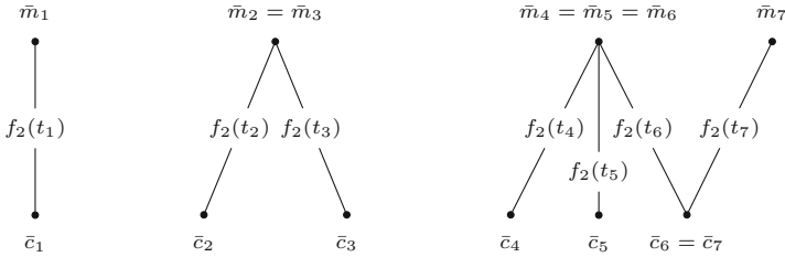
Fig. 3. Example of a bipartite graph G representing seven evaluations of \text{GCL}^{f_1, f_2, f_3} . For brevity, we denote \tilde{m}_i = m_i \oplus f_1(t_i) and \tilde{c}_i = c_i \oplus f_3(t_i) . Graph view rotated for economical reasons.
