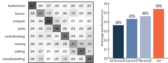
Figure 5. Comparison of classification results. Left: Overall performance. Confusion table for the 8-way scene classification. Rows represent the models for each scene while the columns represent the ground truth classes. The overall classification performance is 54%. Right: Comparison with different models (Experiment A). Performance of four methods. Percentage on each bar represents the average scene classification performance. 3rd bar is the modified Corr-LDA model [3].
