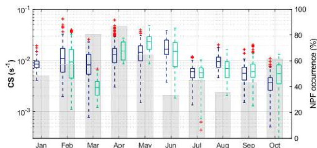
Figure 14. Monthly variation of condensation sink ( s^{-1} ) during event (blue) and non-event (green) days using data corresponding to when global radiation is greater than 50 \text{ W m}^{-2} . The bottom and top edges of the boxplots indicate the 25th and 75th percentiles, respectively. The central mark indicates the median. The whiskers extend to the most extreme data points not considered outliers, and the outliers are plotted individually using the “+” symbols. Data presented have hourly time resolution. The shaded grey bars represent the monthly NPF percent occurrence.
