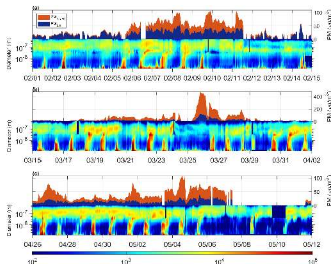
Figure 10. Temporal variations of aerosols during dust episodes with 5 d before and 5 d after the dust episode. (a) Time series of particle size distribution, \text{PM}_{10-2.5} , and \text{PM}_{2.5} between 1 and 15 February 2018 (dust episode: 6 to 10 February). (b) Time series of particle size distribution, \text{PM}_{10-2.5} , and \text{PM}_{2.5} between 15 March and 2 April 2018 (dust episode: 20 to 28 March). (c) Time series of particle size distribution, \text{PM}_{10-2.5} , and \text{PM}_{2.5} between 26 April and 15 May 2018 (dust episode: 26 to 27 April and 1 to 7 May).
