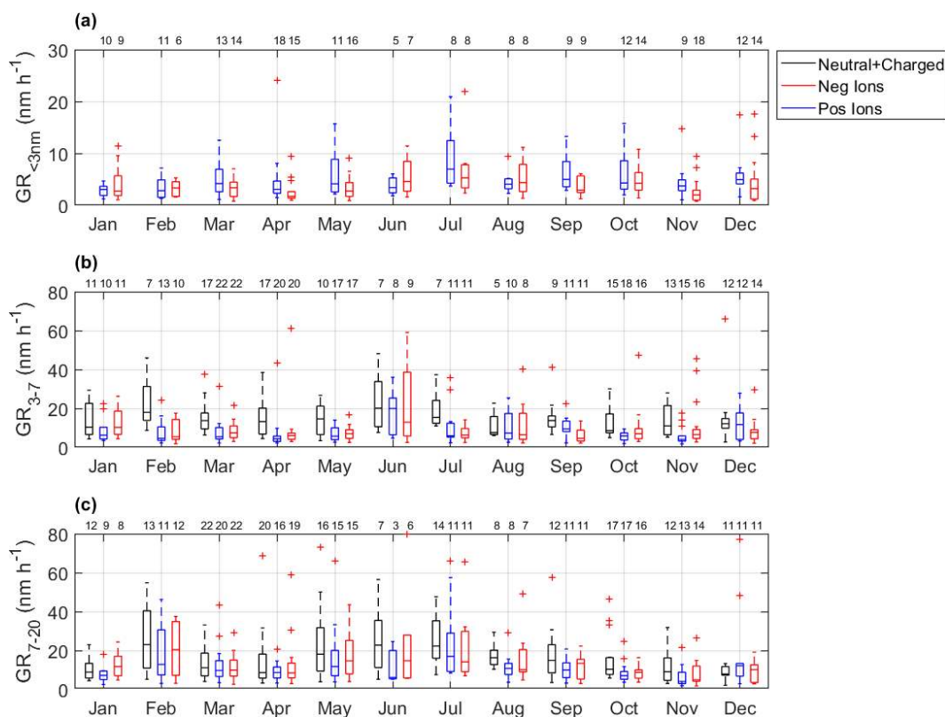
Figure 13. Monthly variation of growth rates during NPF events in three size ranges: (a) < 3 nm, (b) 3–7 nm, and (c) 7–20 nm. The central marks indicate the median, and the bottom and top edges of the boxes indicate the 25th and 75th percentiles, respectively. The whiskers extend to the most extreme data points not considered outliers, and the outliers are plotted individually using the “+” symbols. The numbers above the boxplot represent the number of data points within each boxplot. Black boxes represent the total particles (neutral+charges), blue boxes represent negative ions, and red boxes represent positive ions.
