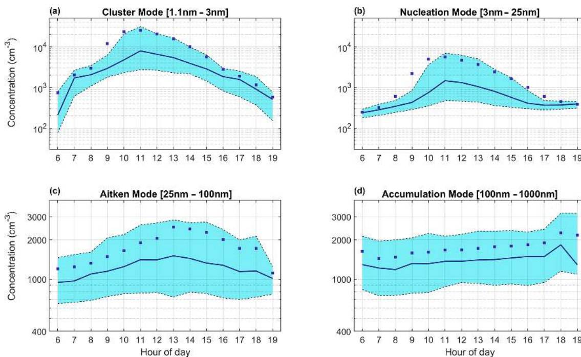
Figure 3. The diurnal cycle (at radiation > 50 \text{ W m}^{-2} ) of particle number concentration of cluster mode (a), nucleation mode (b), Aitken mode (c), and accumulation mode (d). The shaded areas with dashed black boundaries represent the 25th and 75th percentile limits, while the solid line represents the median and the squares indicate the mean. Notice the difference in the y scale between the top and bottom plots.
