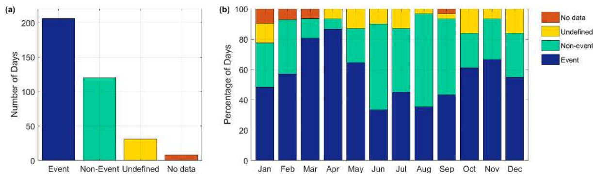
Figure 4. Classification of NPF events presented (a) annually and (b) monthly.
