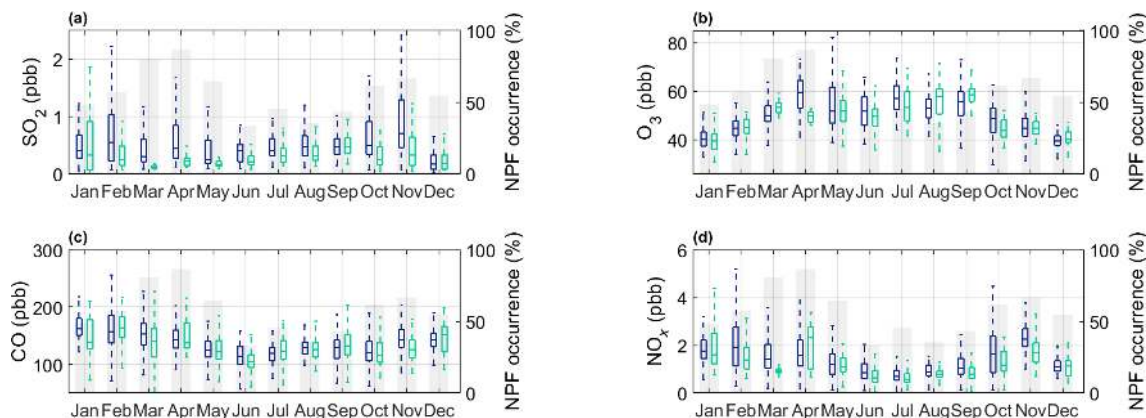
Figure 16. Monthly variation of trace gases during event (blue) and non-event (green) days: (a) sulfur dioxide, (b) ozone, (c) carbon monoxide, and (d) nitrogen oxides using data corresponding to days when global radiation was greater than 50 \text{ W m}^{-2} . The shaded grey bars represent the monthly NPF percent occurrence. The bottom and top edges of the boxplots indicate the 25th and 75th percentiles, respectively. The central mark indicates the median. The whiskers extend to the most extreme data points not considered outliers. Data presented have hourly time resolution. The shaded grey bars represent the monthly NPF percent occurrence.
