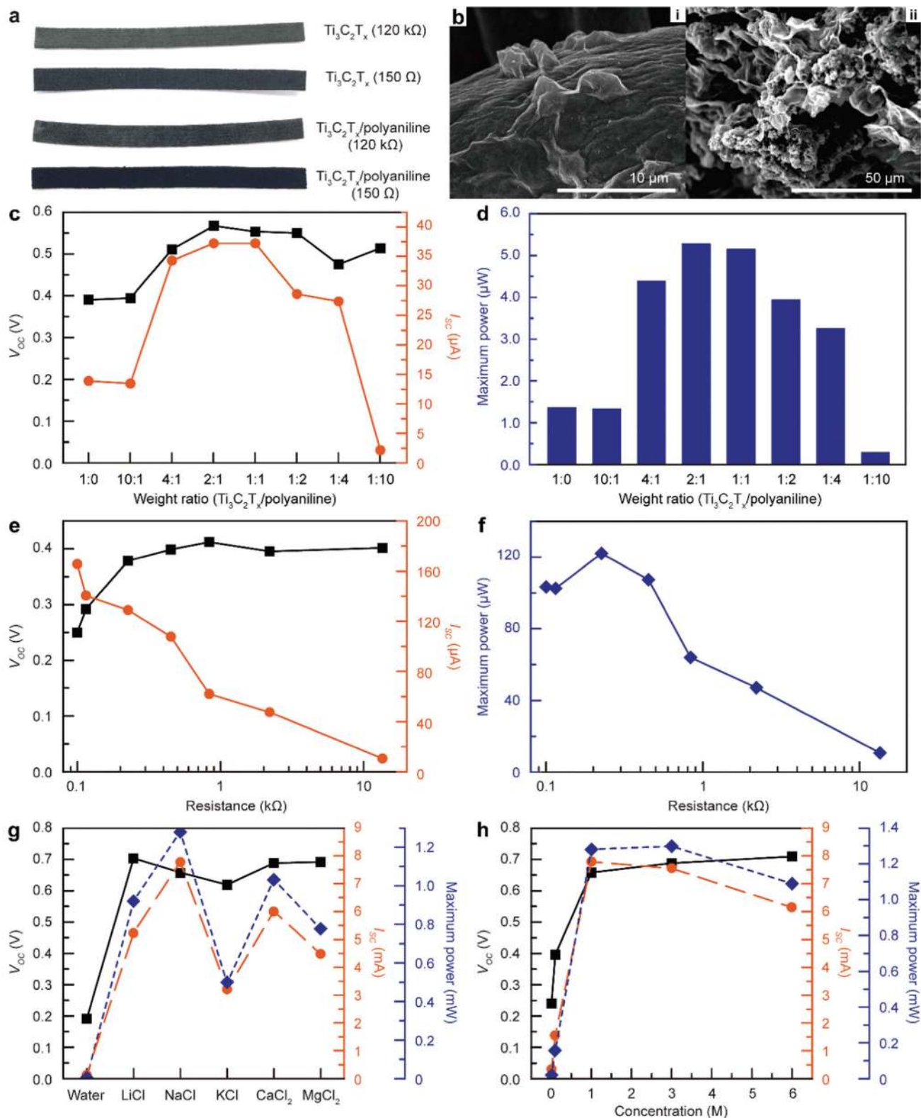
Fig. 4 Energy generation performance of \text{Ti}_3\text{C}_2\text{T}_x/\text{polyaniline} -based TEPG (MPTEPG). (a) Photographic images of MTEPG and MPTEPG with resistances of 150 \Omega and 120 k \Omega . (b) SEM images of MPTEPG. i and ii are a front view and a cross-sectional view of \text{Ti}_3\text{C}_2\text{T}_x/\text{polyaniline} -coated cotton fiber, respectively. (c) Measured V_{\text{oc}} and I_{\text{sc}} values from the MPTEPG (250 \Omega ) with various polyaniline contents. (d) Measured power from the MPTEPG (250 \Omega ) with various polyaniline contents. (e) Measured V_{\text{oc}} and I_{\text{sc}} values from the MPTEPG with various bulk resistance. (f) Generated power from the MPTEPG (weight ratio 1:1, 250 \Omega ) as a function of bulk resistance. (g) Measured V_{\text{oc}} , I_{\text{sc}} , and power values from the MPTEPG (weight ratio 1:1, 250 \Omega ) with various electrolyte solutions (1 M). (h) Measured V_{\text{oc}} , I_{\text{sc}} , and power values from the MPTEPG (weight ratio 1:1, 250 \Omega ) with NaCl solution of various concentrations.
