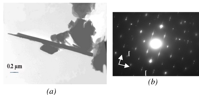
Figure 4: (a) Transmission electron image of antigorite fibrils as seen perpendicularly to fibre axis, i.e. [001] crystallographic direction. (b) Selected area electron diffraction from a sample shown in (a) taken along the same crystallographic direction.
